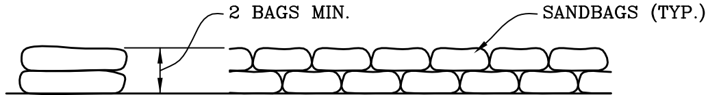
TYPICAL SECTION
